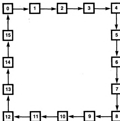
÷ 16 STATE DIAGRAM
