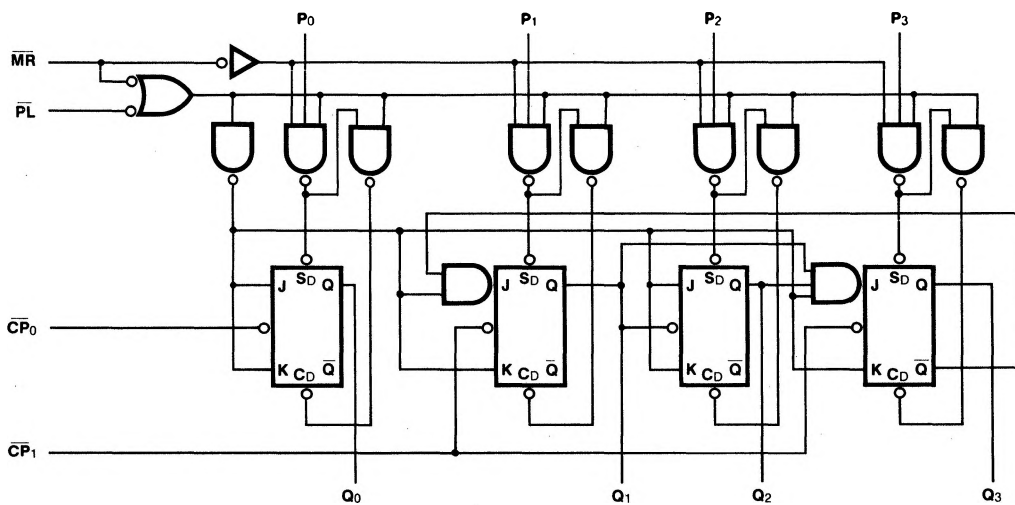
LOGIC DIAGRAM
