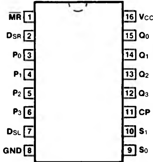
CONNECTION DIAGRAM PINOUT A
