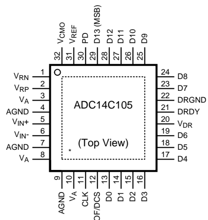
Figure 1. WQFN Package See Package Number RTV0032A
