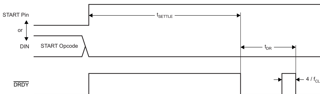
Figure 32. Settling Time
