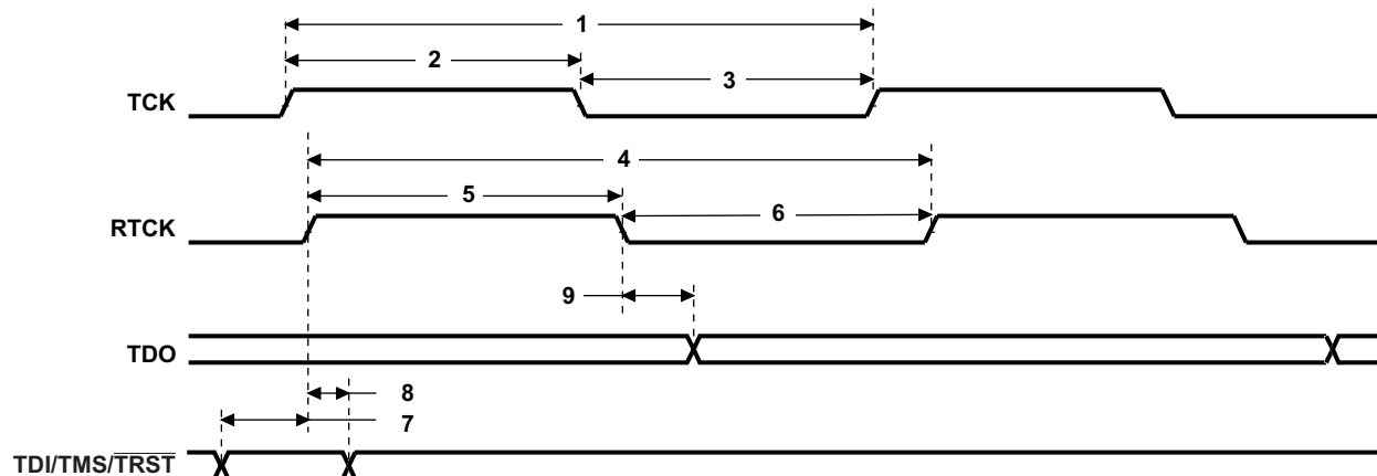
Figure 5-81. JTAG Test-Port Timing
