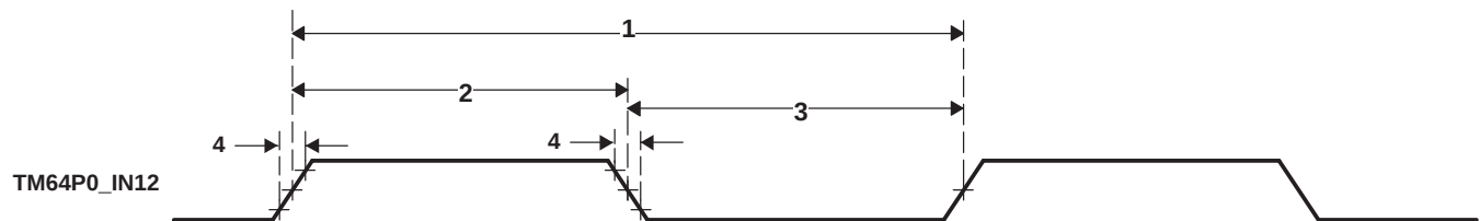
Figure 5-72. Timer Timing
