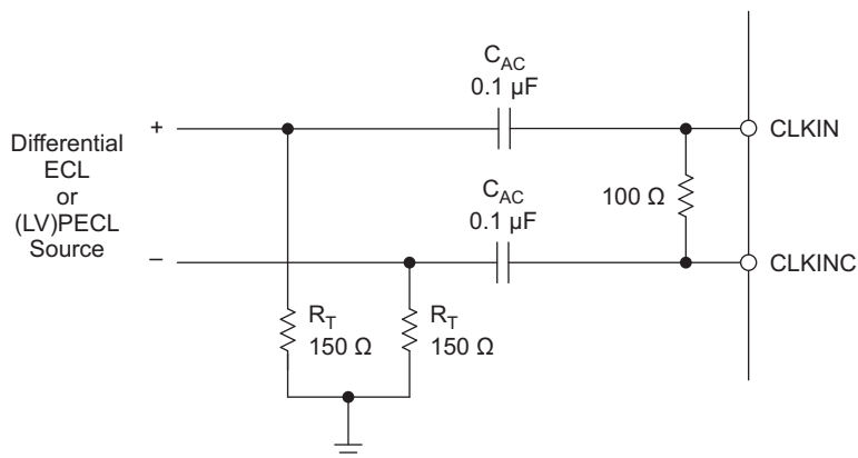
Figure 83. Preferred Clock Input Configuration with a Differential ECL/PECL Clock Source
