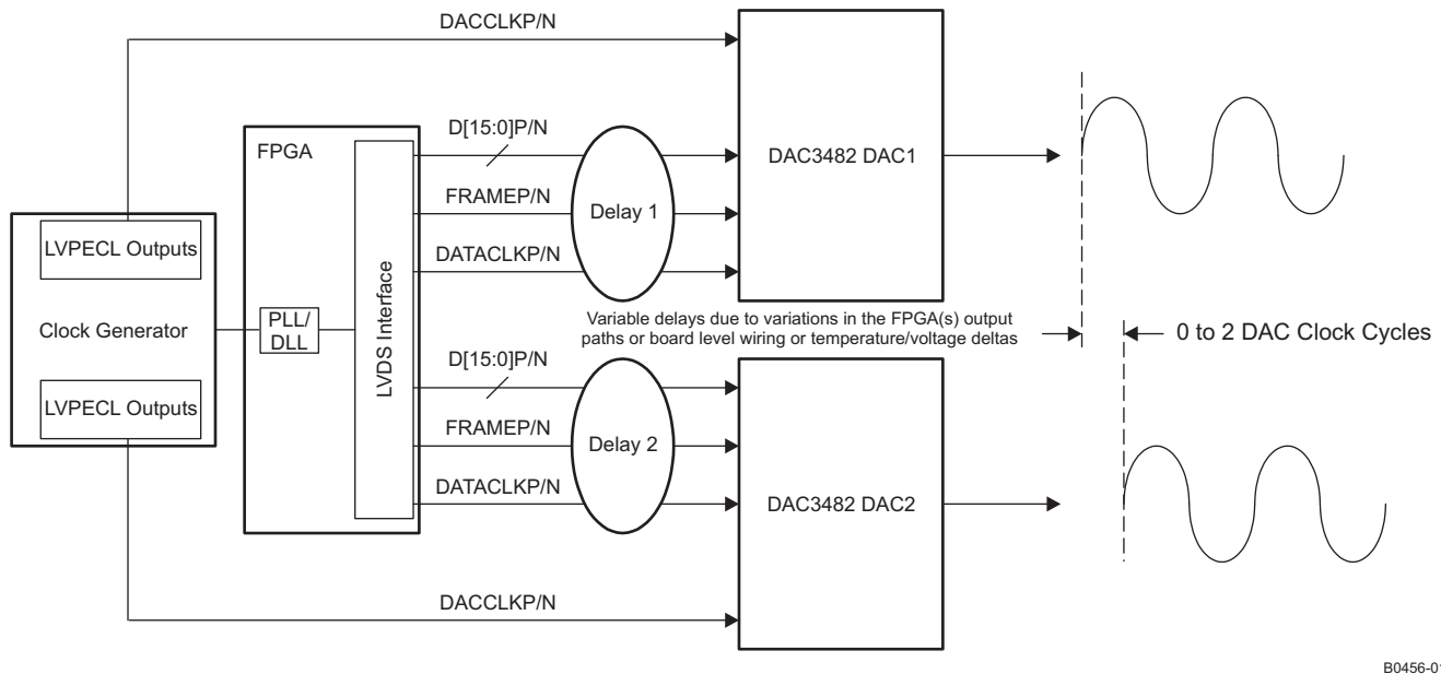
Figure 62. Multi-Device Operation in Single Sync Source Mode
