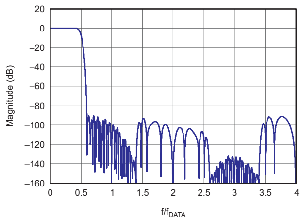
Figure 69. 8x Interpolation Composite Response
