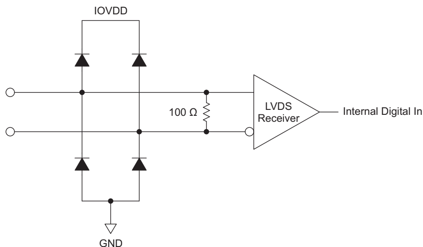
Figure 84. D[15:0]P/N, DATACLKP/N, FRAMEP/N, SYNCN/P and PARITYP/N LVDS Input Configuration
