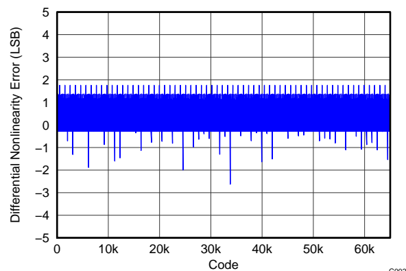
Figure 2. Differential Nonlinearity
