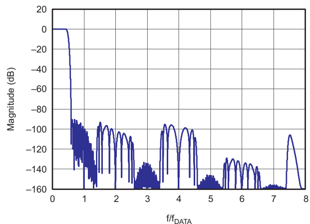
Figure 70. 16x Interpolation Composite Response
