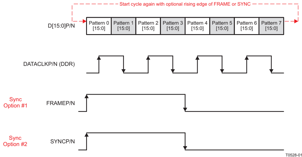
Figure 78. IO Pattern Checker Data Transmission Format
