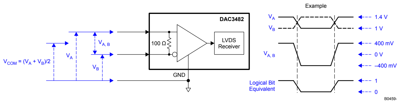
Figure 85. LVDS Data Input Levels
