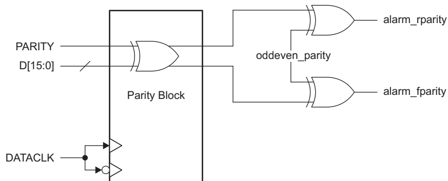
Figure 80. DAC3482 Word-by-Word Parity Check
