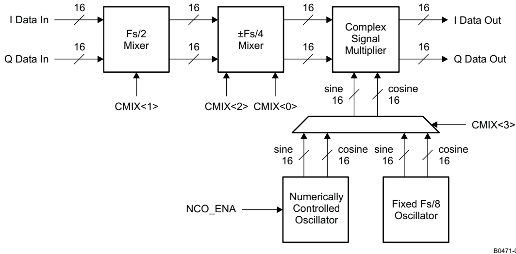
Figure 72. Path of Complex Signal Mixer
