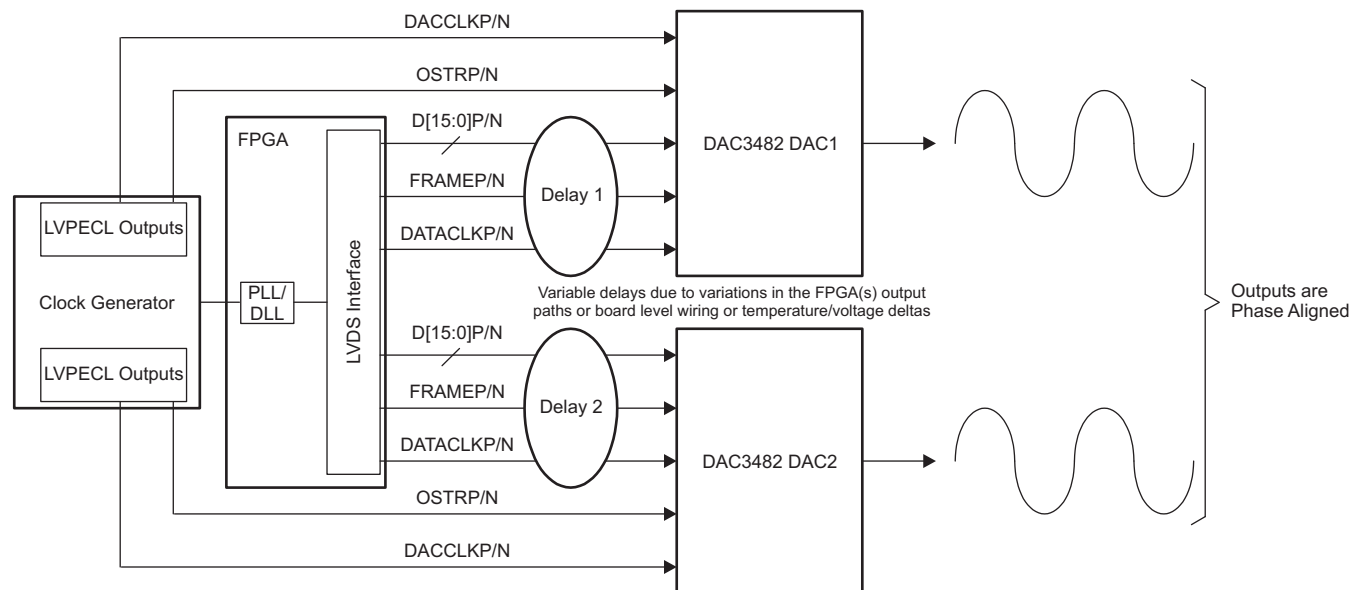
Figure 59. Synchronization System in Dual Sync Sources Mode with PLL Bypassed
