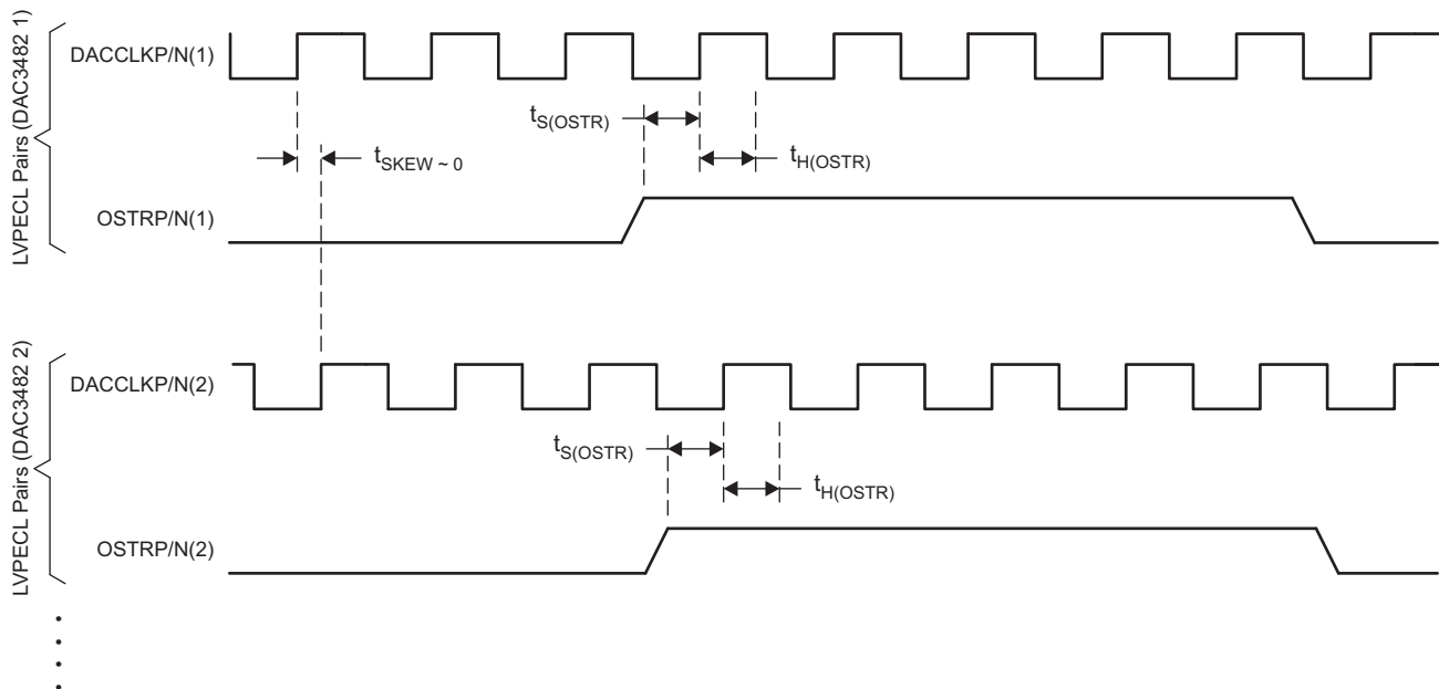
Figure 60. Timing Diagram for LVPECL Synchronization Signals
