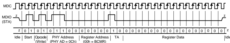
Figure 2-6. Typical MDC/MDIO Write Operation
