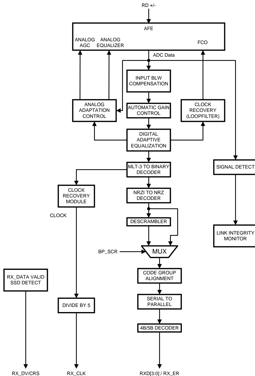
Figure 2-8. 100BASE-TX Receive Block Diagram
