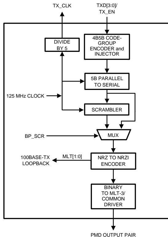
Figure 2-7. 100BASE-TX Transmit Block Diagram
