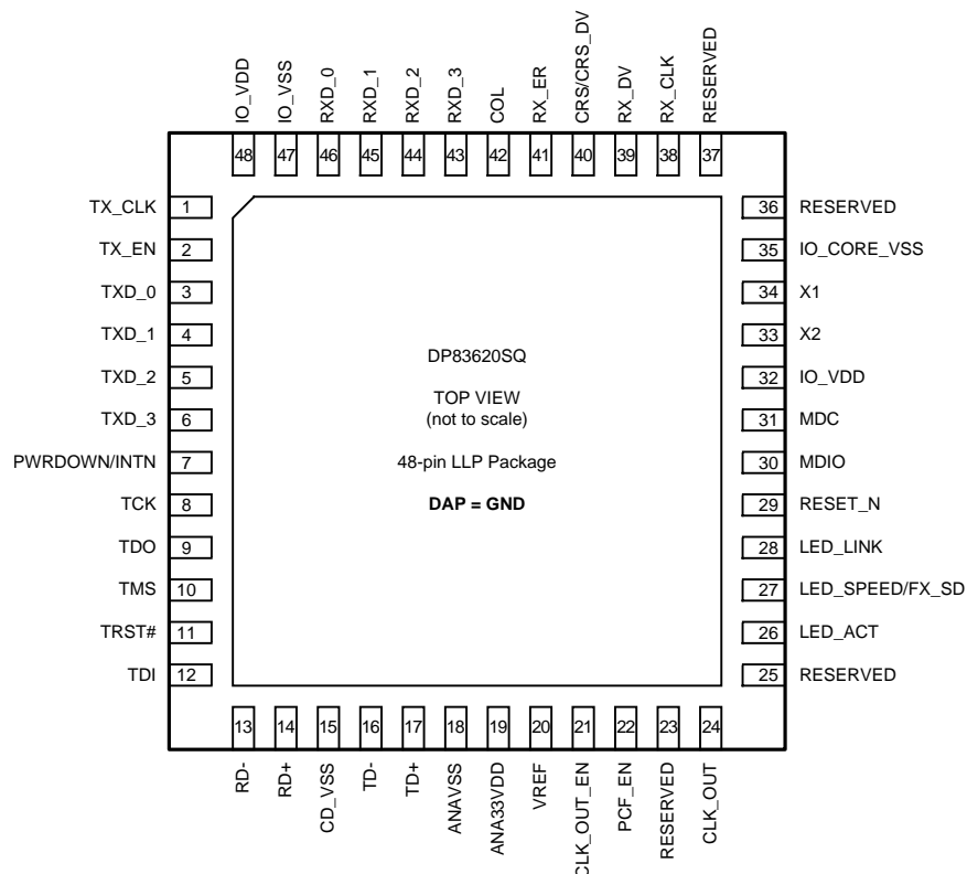
Figure 2-2. Top View Package Number RHS0048A
