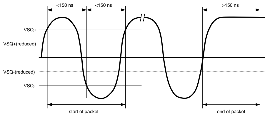
Figure 2-9. 10BASE-T Twisted Pair Smart Squelch Operation
