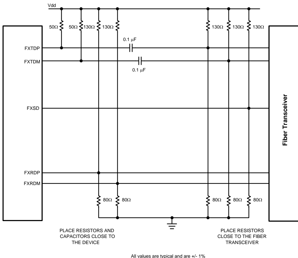
Figure 2-11. 100 Mb/s Fiber Pair Interface
