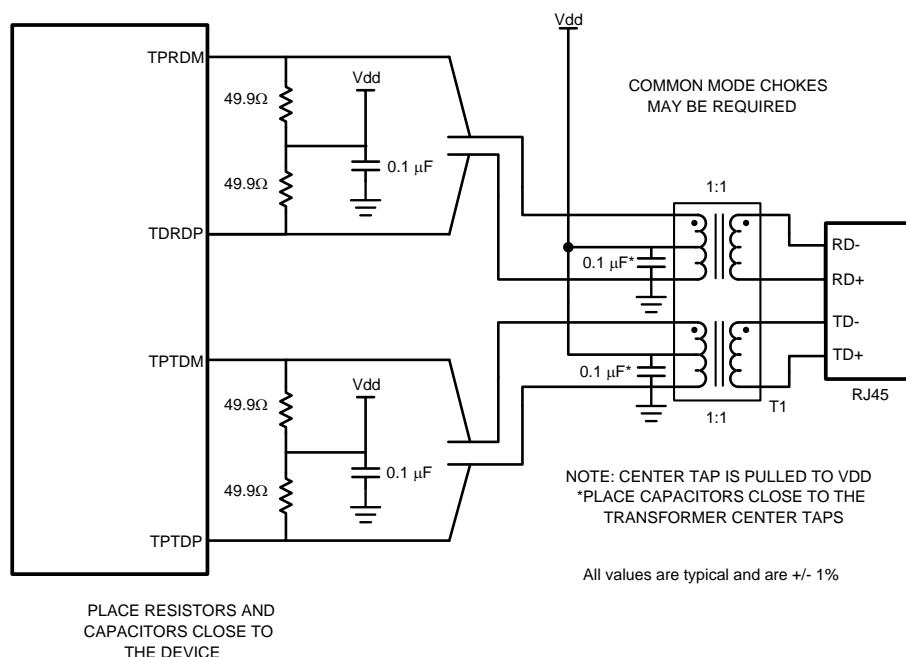
Figure 2-10. 10/100 Mb/s Twisted Pair Interface
