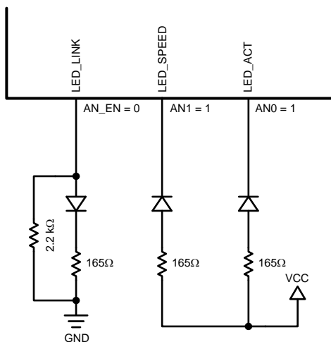
Figure 2-4. AN Strapping and LED Loading Example
