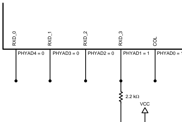
Figure 2-3. PHYAD Strapping Example
