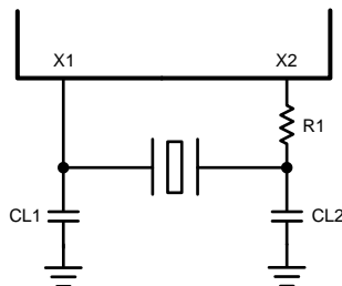
Figure 2-12. Crystal Oscillator Circuit
