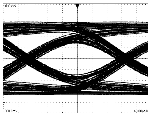
Figure 21. A 3.125 Gbps NRZ PRBS-7 with PE After 40\"
