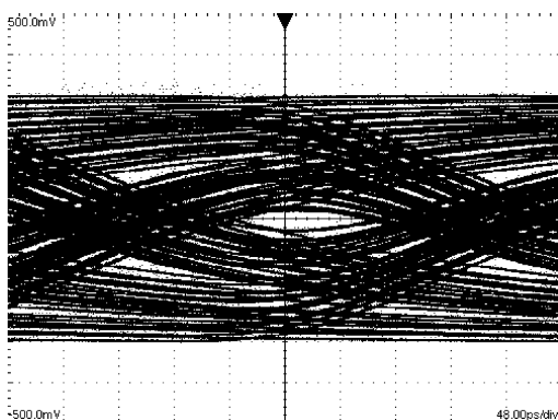
Figure 20. A 3.125 Gbps NRZ PRBS-7 without PE or EQ After 40\"
