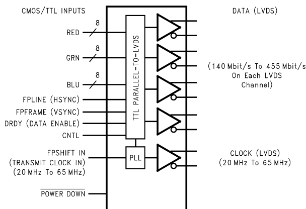
Figure 1. DS90C383B
