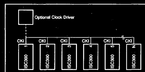
FIGURE 6. Synchronizing Multi-ISC300 Applications.
