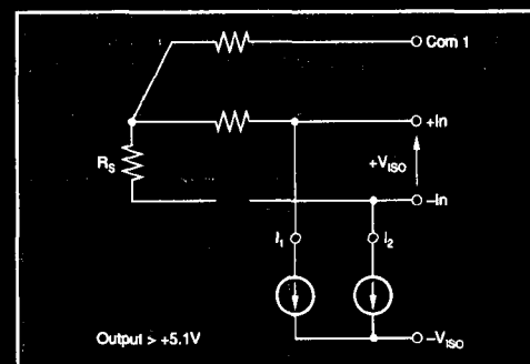
FIGURE 12. -In Open Circuit.
