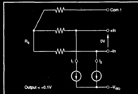
FIGURE 10. R_S Short Circuit.
