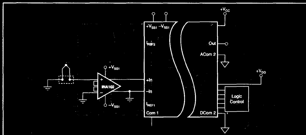
FIGURE 18. Temperature Measurement Using Thermocouple with Small Span.
