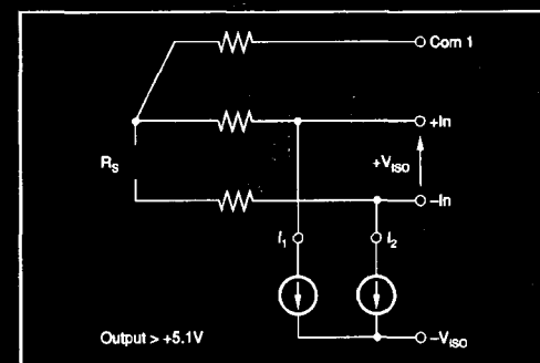
FIGURE 9. R_S Open Circuit.
