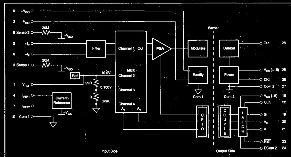
FIGURE 1. ISC300 Block Diagram.
