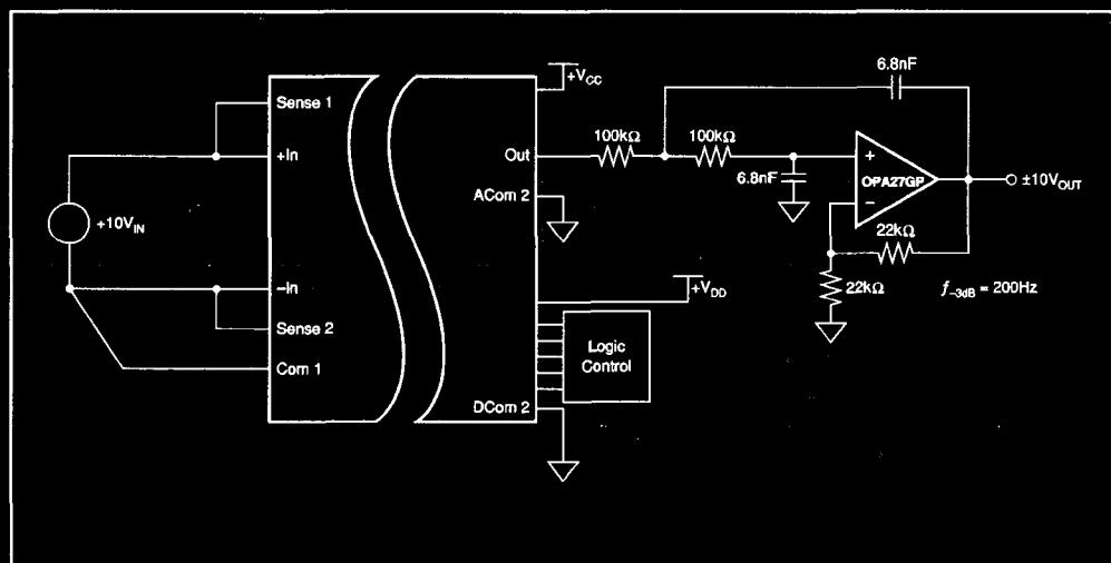
FIGURE 15. Isolated Voltage Measurement Channel with Output Filter.
