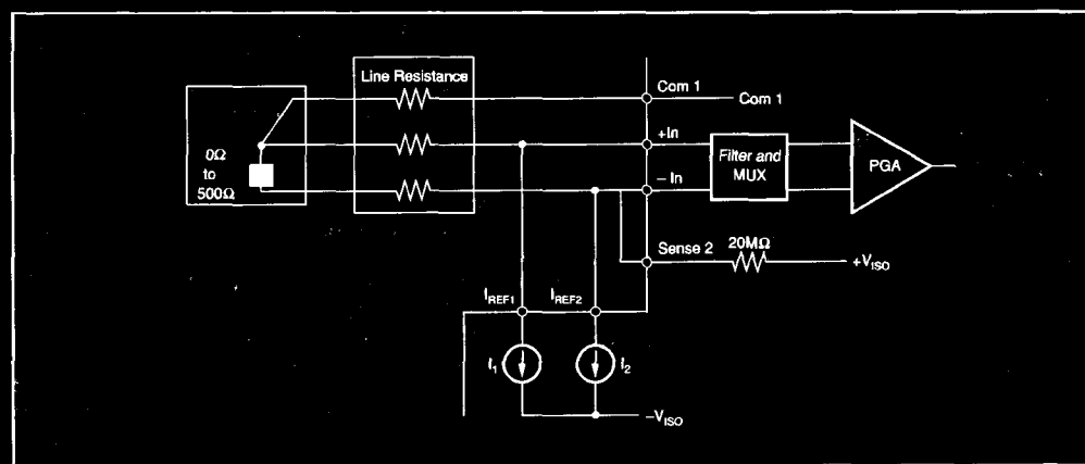
FIGURE 3. Resistance Measurement Configuration.
