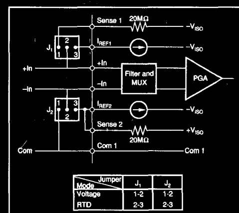
FIGURE 7. Mode Selection Jumpers.
