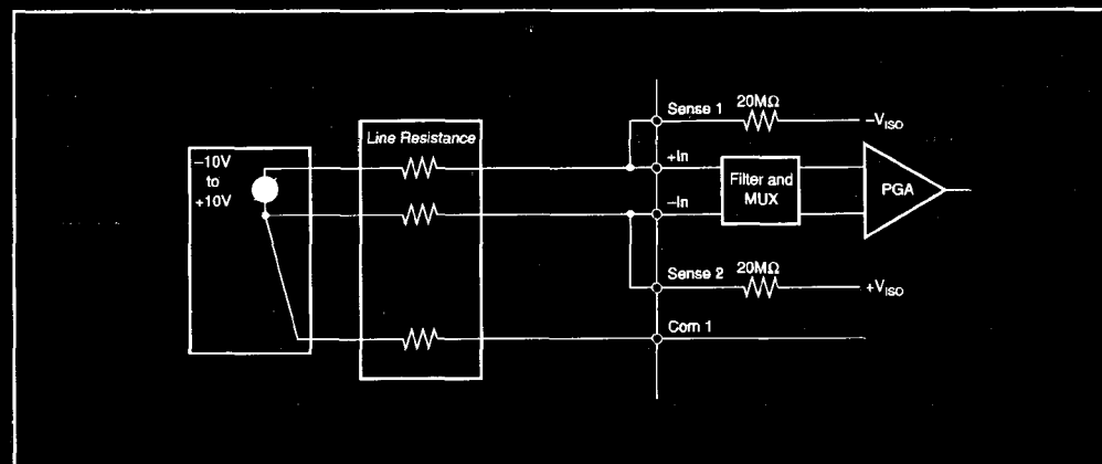
FIGURE 4. Voltage Measurement Configuration.
