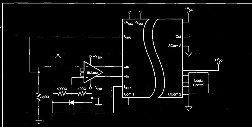
FIGURE 19. Thermocouple with Cold Junction Compensation.
