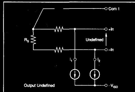
FIGURE 14. Com 1 Open Circuit.
