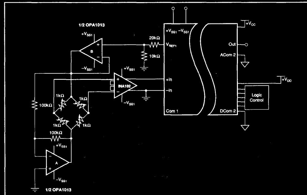
FIGURE 16. Isolated Instrument Bridge System.
