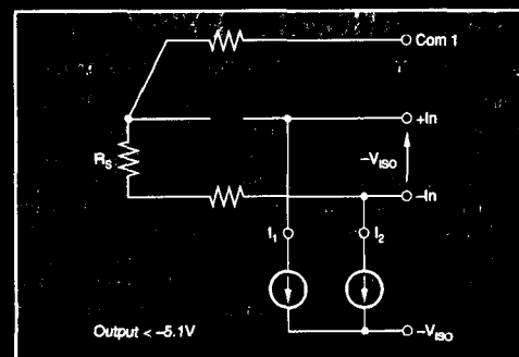
FIGURE 11. +In Open Circuit.
