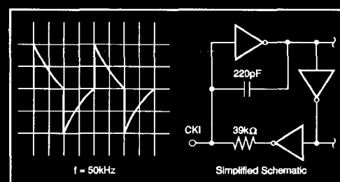
FIGURE 5. CKI Input.
