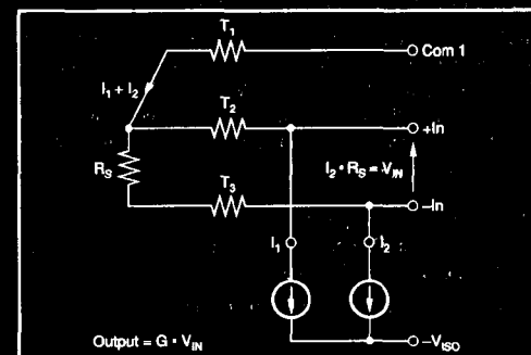
FIGURE 8. Normal Operation.
