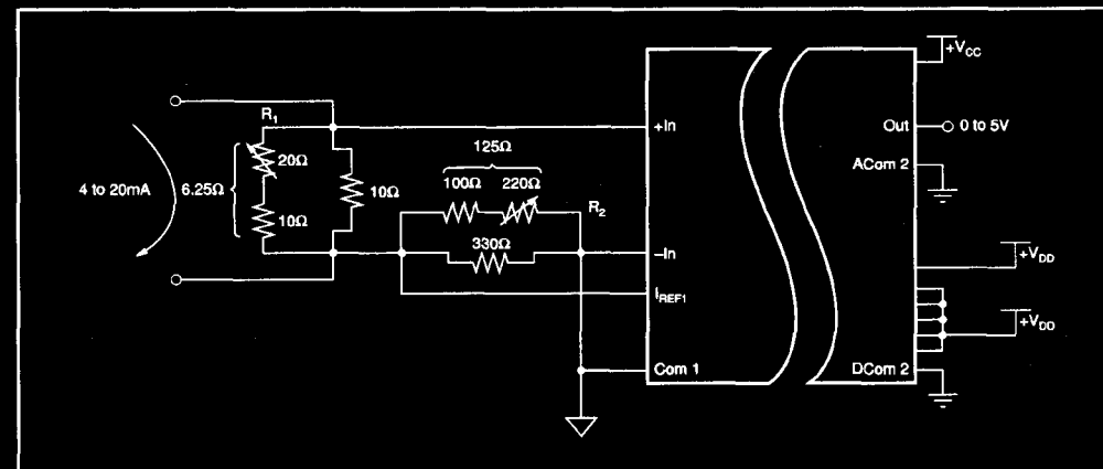
FIGURE 17. Isolated 4 to 20mA receiver (0 to 5V output).
