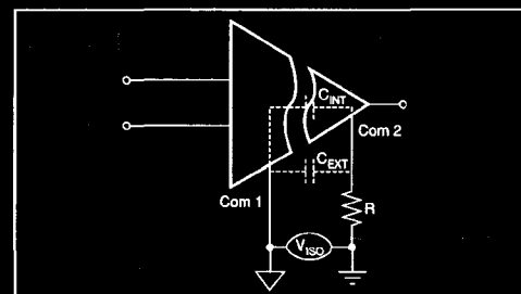
FIGURE 2. Barrier Capacitance.
