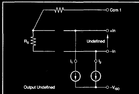
FIGURE 13. -In and +In Open Circuit.
