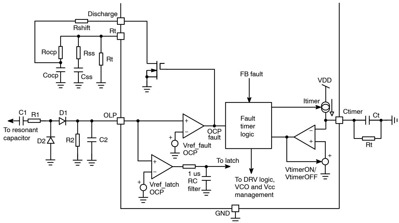
Figure 40. Overload Protection Input Connection NCP1398B
