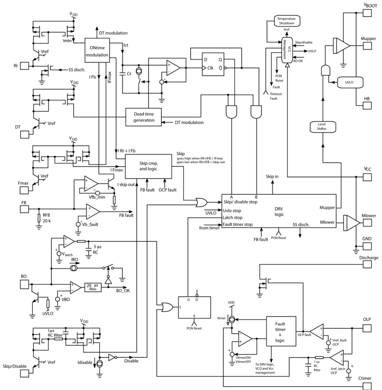
Figure 2. Internal Circuit Architecture – NCP1398C
