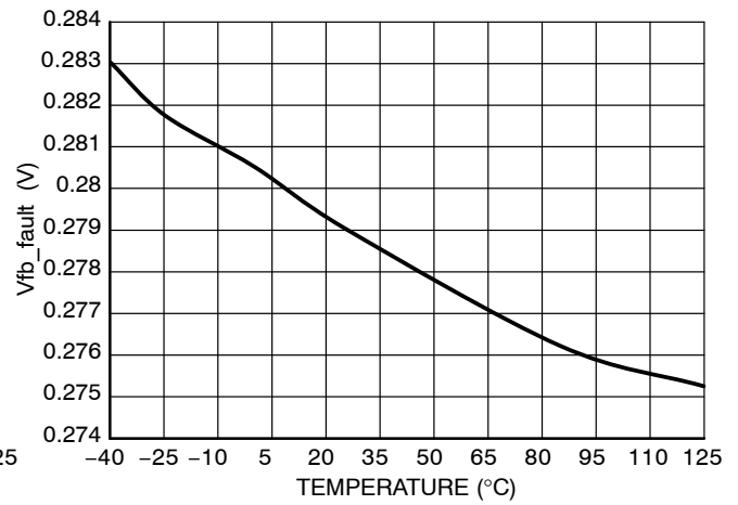
Figure 9. FB Fault Reference (Vfb_Fault)
