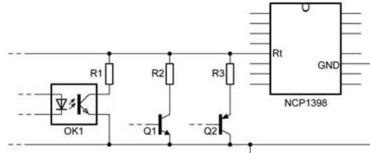
Figure 31. Other Possibilities How to Modulate Operating Frequency of the NCP1398 Using Direct Connection to Rt Pin
