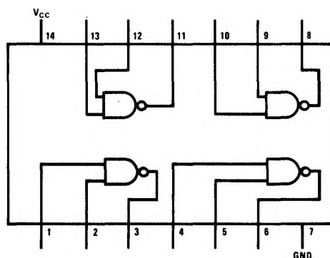
DM5403/DM7403
