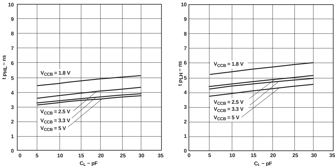
Figure 4. TYPICAL PROPAGATION DELAY (B to A) vs LOAD CAPACITANCE
