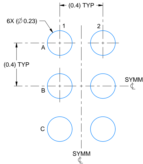
LAND PATTERN EXAMPLE EXPOSED METAL SHOWN SCALE:50X
